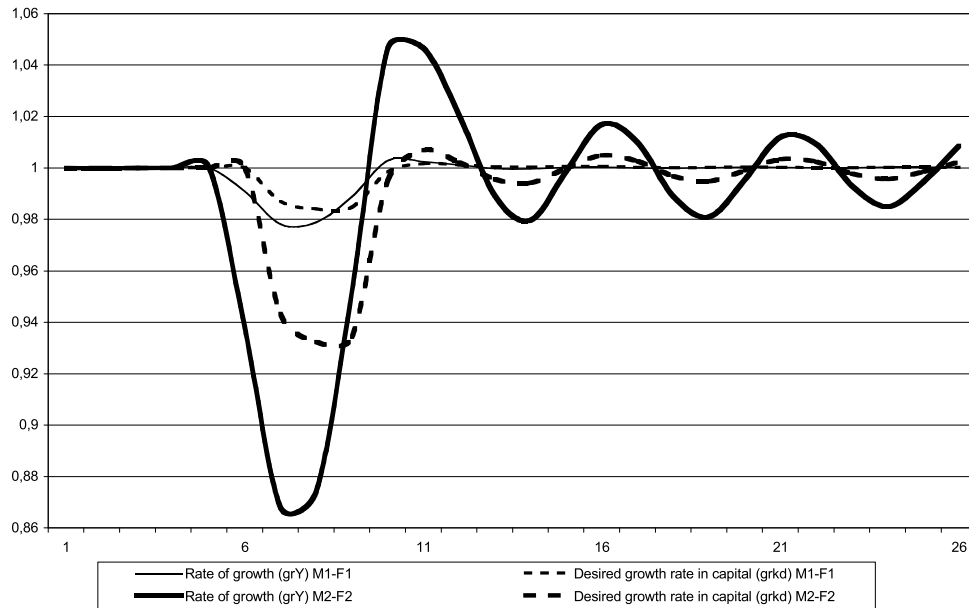
Figure 8.3 Inflationary shock of 1 % during 3 years (M1-F1, M2-F2): effects on the growth rate of the economy and on the desired rate of accumulation
