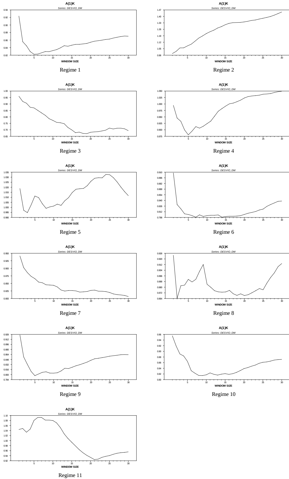
Figure A.2: Temporal Permanence of a Unit Shock in the Context of the Cochrane and Campbell Test (Regimes 1 to 11)
