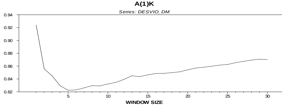
Figure 4: Temporal Permanence of a Unit Shock in the Context of the Cochrane and Campbell Test (Regime 1)
